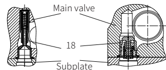
Model 4WEH16...-7X/.../P4.5 Model 4WEH25.../.../P4.5 Model 4WEH32.../.../P4.5
