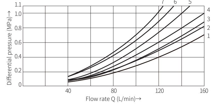
Model 4WEH10...(Measured at \nu_{oil}=41\text{mm}^2/\text{s} and t=50^\circ\text{C} )
