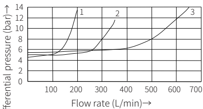
Model 4WEH16...-7X/.../P4.5 Model 4WEH25.../.../P4.5 Model 4WEH32.../.../P4.5
